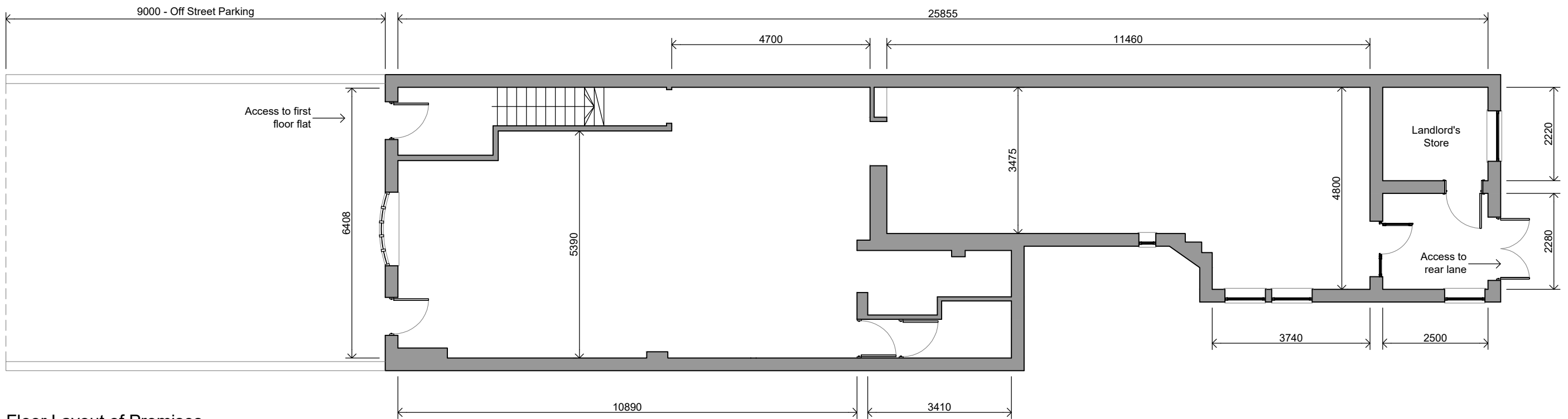
Floor Layout of Premises
